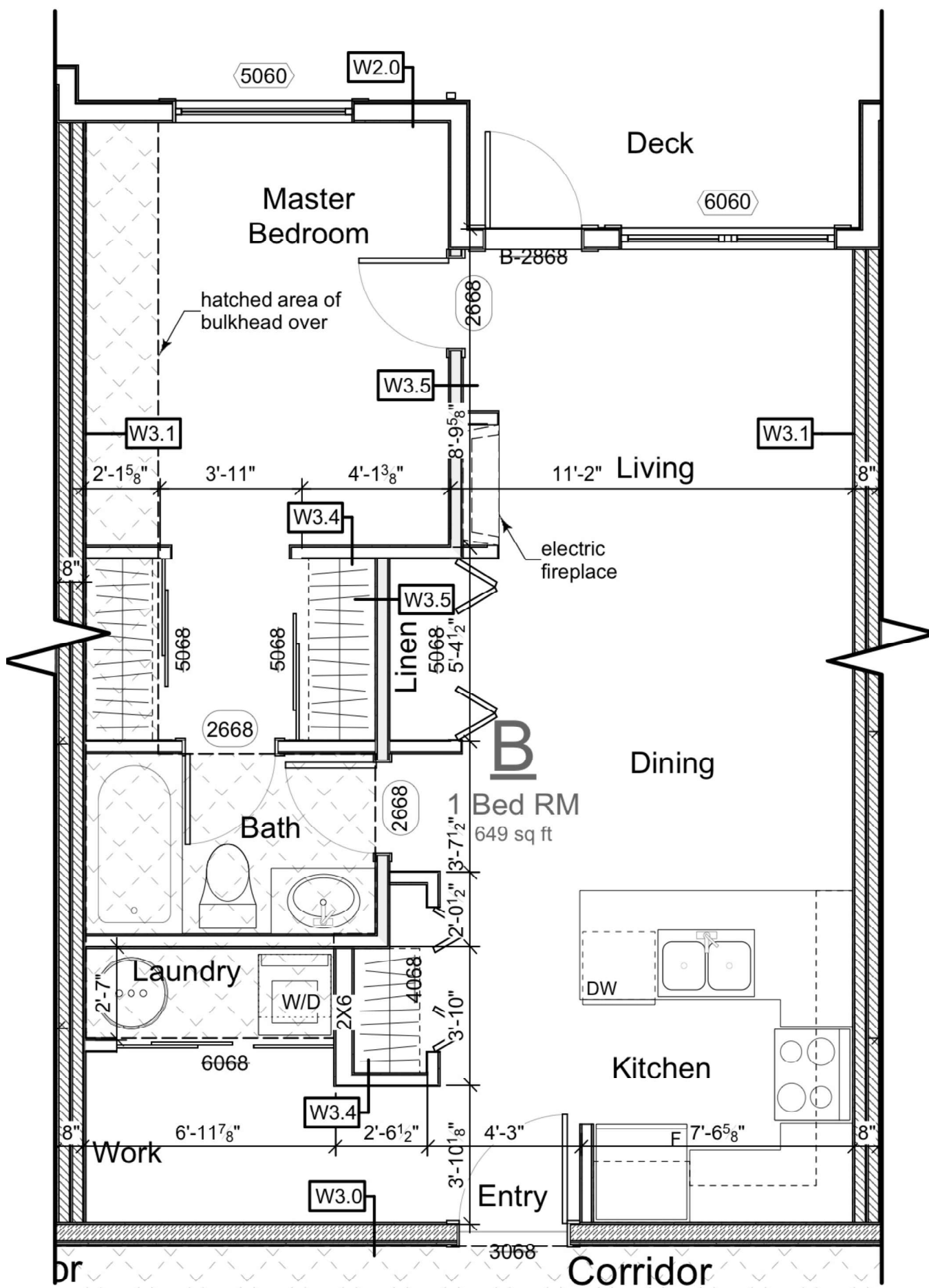
Unit B Layout
