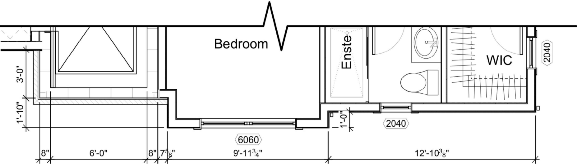
Unit H3 Layout Scale: 1/4" = 1'-0"
