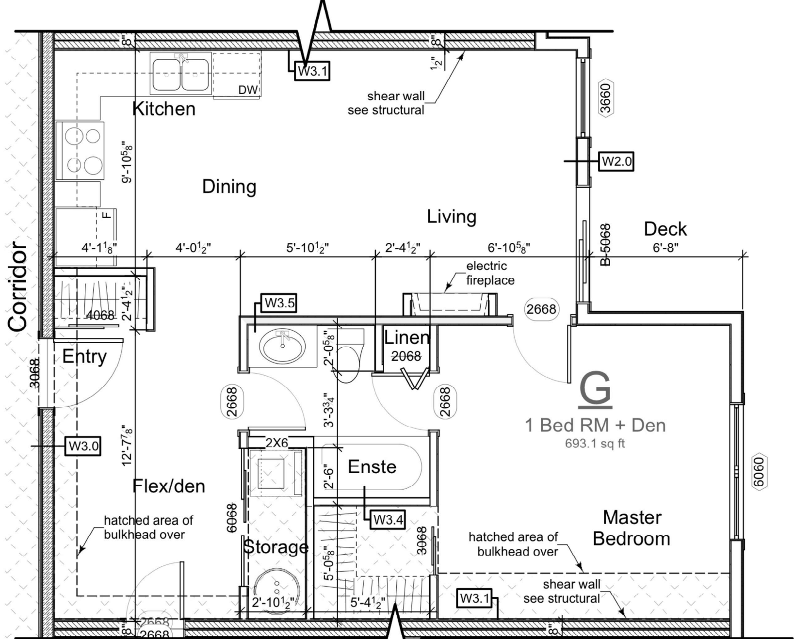
Unit F Layout
